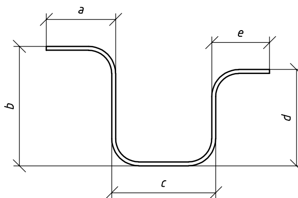
Figure 3 — Bending dimensions — Shape code 25
